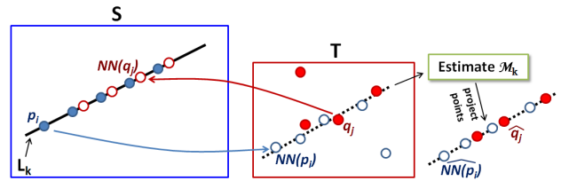
Figure 7: Model constraints. L_k is a straight line in the source image S . For point p_i on L_k , the nearest neighbor in T is NN(p_i) . A point q_i in T has nearest neighbor NN(q_i) that lies on L_k . We collect all such points NN(p_i) and q_i and robustly compute the best line M_k in T , then project the points to the estimated line.
